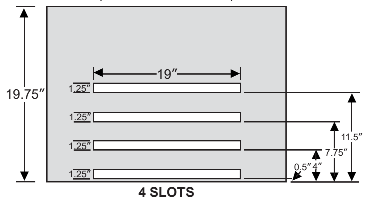
REAR VIEW (inside dimensions)
