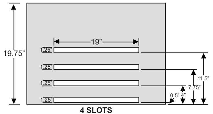
REAR VIEW (inside dimensions)
