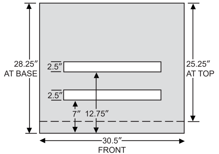
TOP VIEW (inside dimensions)
